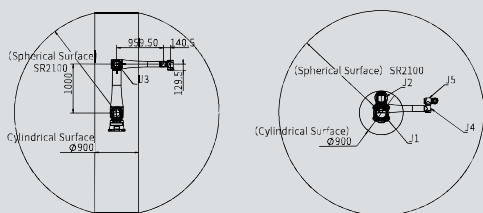
AUBO-iS35 Moving Range of Point P
