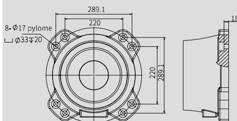
AUBO-iS35 Top View of Base
